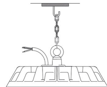
Hoisting chain installation method
